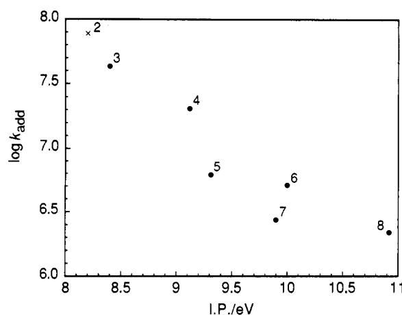
Figure 1. Plot of the log of the rate constants for addition of the perfluoro- n -propyl radical to some alkenes vs ionization potentials of the alkenes. Because the IP for 2 does not reflect the transition-state HOMO (see footnote f in Table I), this point has been indicated by an x.
