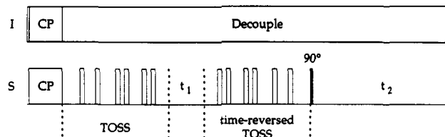
Figure 1. Pulse sequence for a MAS sideband suppression experiment for arbitrary ratios a = \omega_0 \Delta\sigma / \omega_r . Cross polarization is followed by TOSS, an evolution period t_1 , and then time-reversed TOSS. A 90° purging pulse selects one component of the magnetization for detection.
